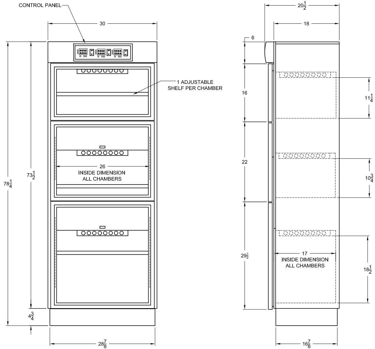
TRIPLE CHAMBER WARMING CABINET TWC24-18
